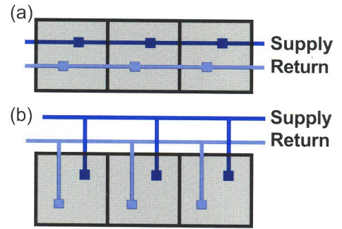
FIGURE 5. Duct Arrangements
