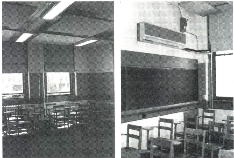
FIGURE 11. Older Classroom Improvements Photograph (a) shows the added sound absorptive material in the form of hanging fabric faced glass fiber panels, wall mounted fabric faced glass fiber panels and carpeting. Photograph (b) shows the relatively noisy wall mounted air conditioning unit with two fan speeds.
