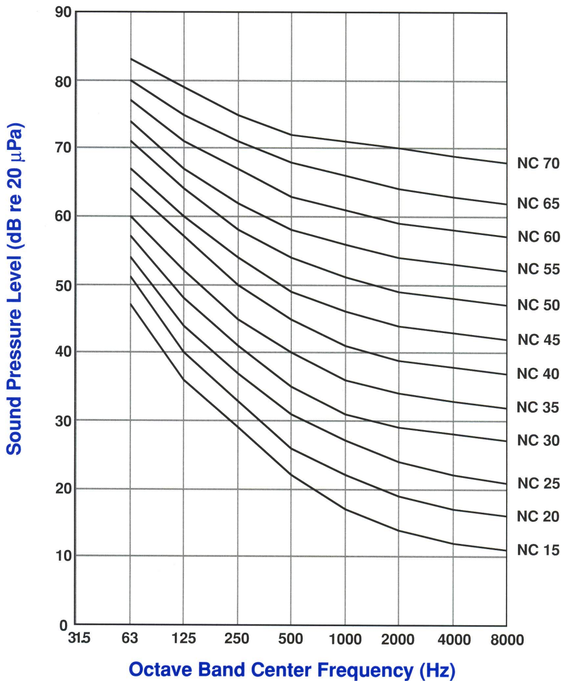
FIGURE 19. Noise Criteria Curve
